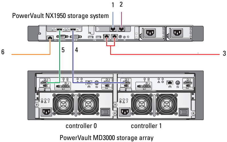
Figure 2-1. Single-Node Configuration
